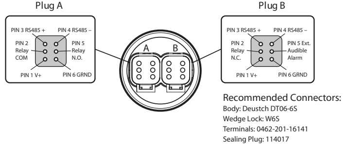
PowerView Audible Alarm Back View Deutsch DT06-6S Style Connections
