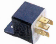
RELAY P/N 405-006-0 12V P/N 405-006-1 24V
